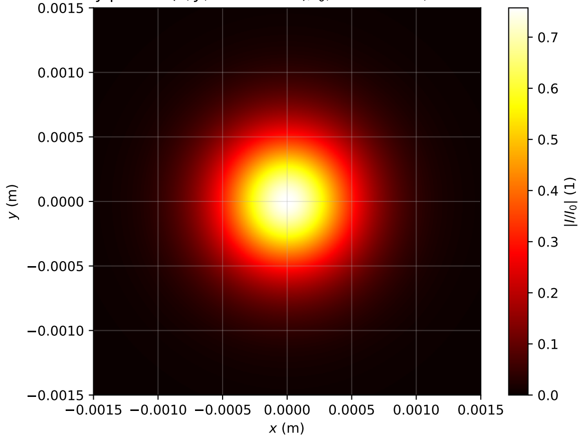
Intensity profile I(x, y, z = 3.344m)/I_0 , P_{in}=0.7P_{cr} , artificial time
